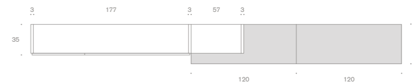
SP025 L/W 423 | H 164 | P/D 35-45
