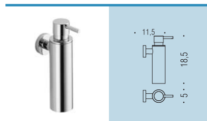
W4981 Spandisapone (L 0,15) Soap dispenser
